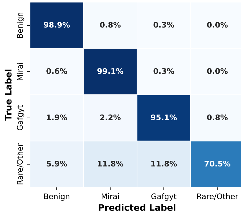
(b) Random Forest
