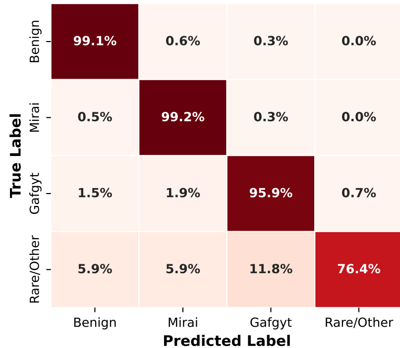
(a) Proposed HolisticELF
